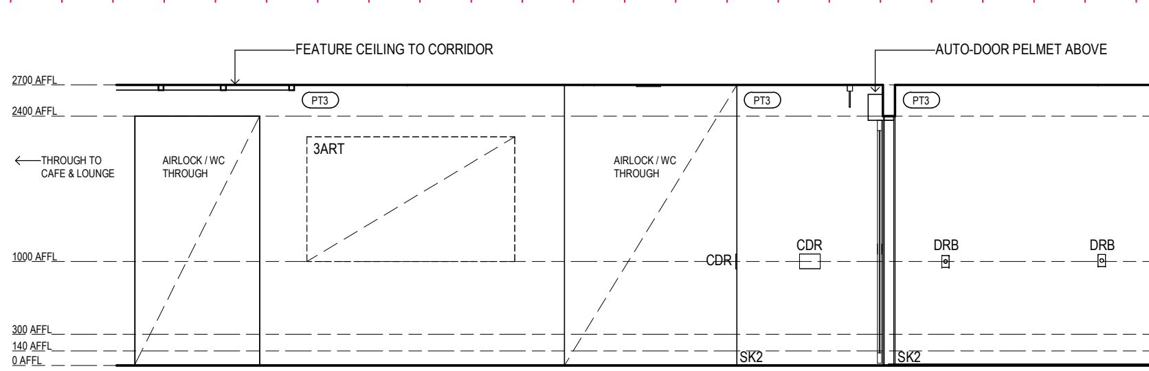
VILLAGE HEALTH & WELLNESS - AIRLOCK & CIRCULATION ELEVATION 1 Scale 1: 50
