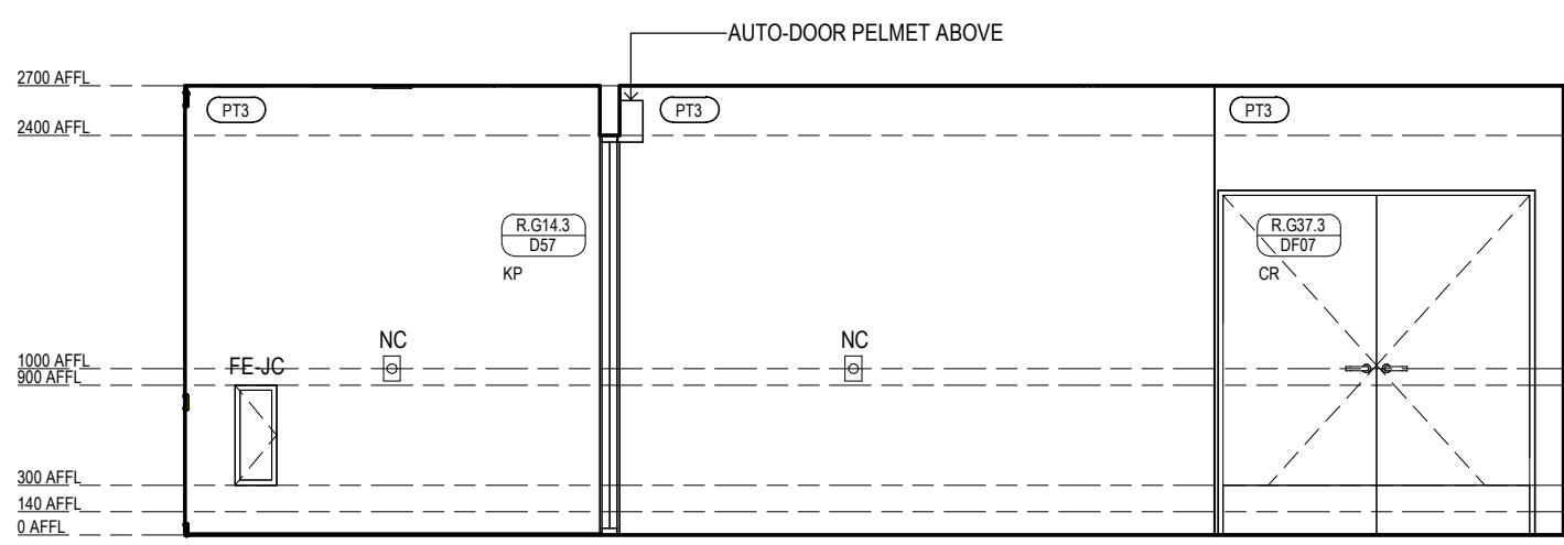
VILLAGE HEALTH & WELLNESS - AIRLOCK & WAITING ELEVATION 2 Scale 1: 50
